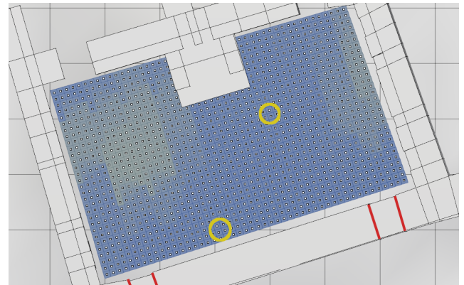
Figure 17: Room 18 heat map showing relative daylight illumination on the floor. This visualizes the annual irradiation at floor node locations. The yellow circles denote the known findspots: [upper right circle] one metal pin, one metal needle, and one stone bead with grooves were found near the hearth at the north side; [lower left circle] one metal bird-shaped object, one metal pin point, five stone beads, and one incised stone bead were found next to the inside south wall in between the two windows.
